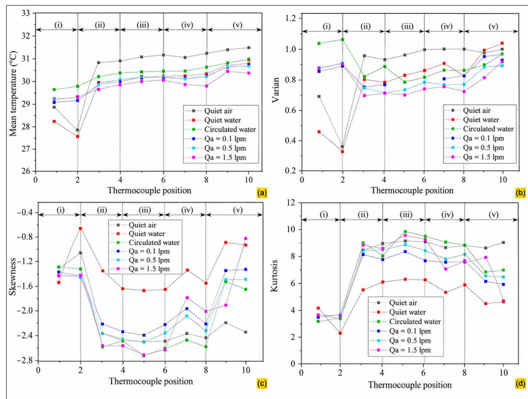
Figure 7. Statistical parameter of temperature: (a) Mean; (b) Varian; (c) Skewness; (d) Kurtosis
