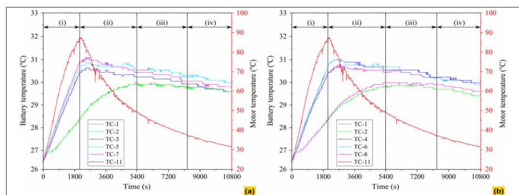
Figure 4. Temperature distribution at Q_a = 0.5 lpm: (a) Time series temperature at left region (TC-3, TC-5, and TC-7); (b) Time series temperature at right region (TC-4, TC-6, and TC-8)
