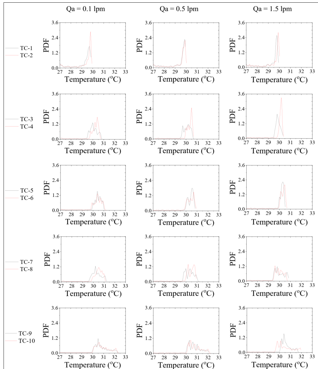
Figure 9. Probability density function for Q_a = 0.1 lpm, 0.5 lpm, and 1.5 lpm
